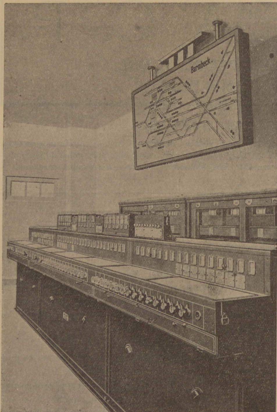
Fig. 1 — Cabine electrica
